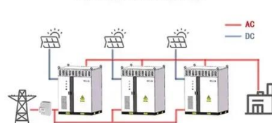
WORKING PRINCIPLE
